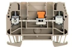
WTL 6/1
