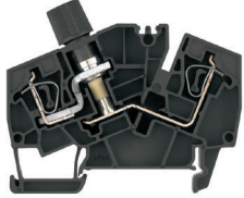
ZSI 2.5-2/2X2AN/G20
